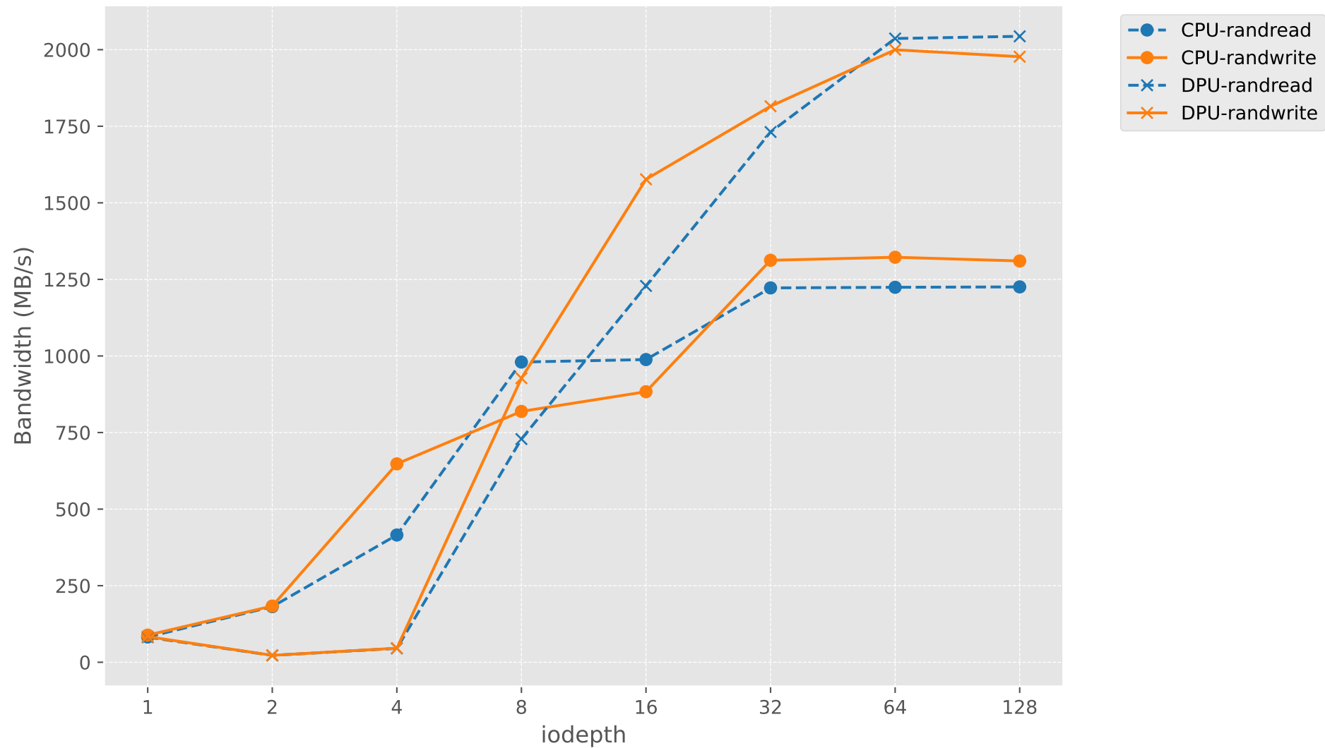
Bandwidth vs iodepth (Random)
